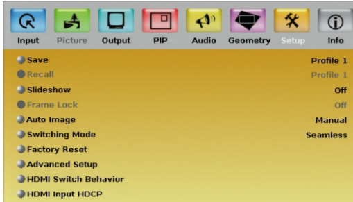
Figure 16: Setup Screen
