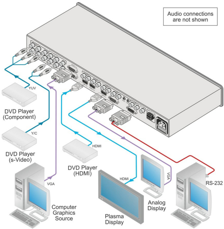
Figure 3: Connecting to the VP-728 Rear Panel
