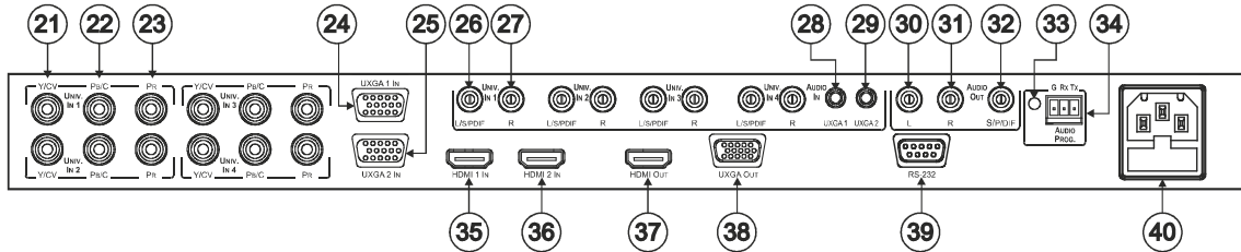
Figure 2: VP-728 Presentation Switcher/Scaler Rear Panel
