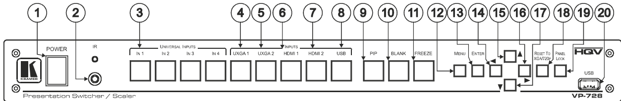
Figure 1: VP-728 Presentation Switcher/Scaler Front Panel
